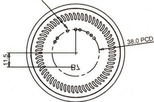
VIEW ON BASE STANDING AREA EMBOSSD WITH CRESCENT STIPPLE
