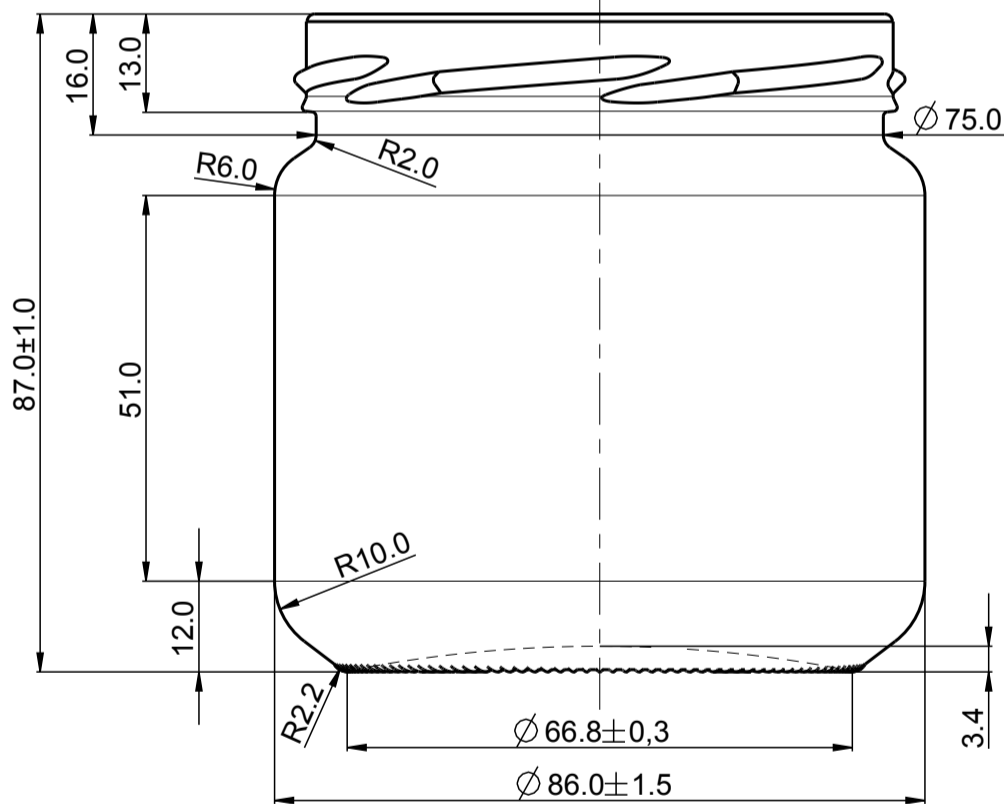
Front view TO 82 CE.T.I.E. GME 20.09:1995 according to FD130
